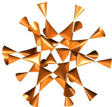
Figure 1: Barth's sextic surface
