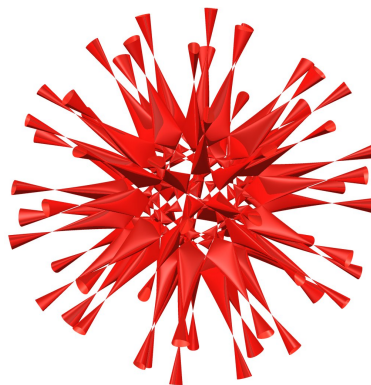
Figure 2: Barth's decic surface
